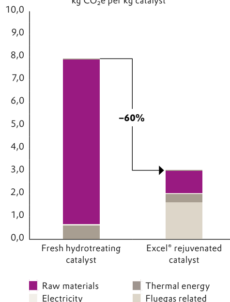
Comparison of greenhouse gas emissions of fresh hydrotreating catalyst versus Excel® rejuvenated catalyst kg CO 2 e per kg catalyst
