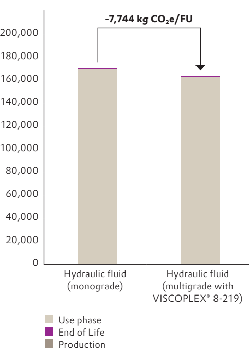
Comparison of greenhouse gas emissions of DYNAVIS® technology and conventional hydraulic fluids (monograde) in mobile construction machinery.
