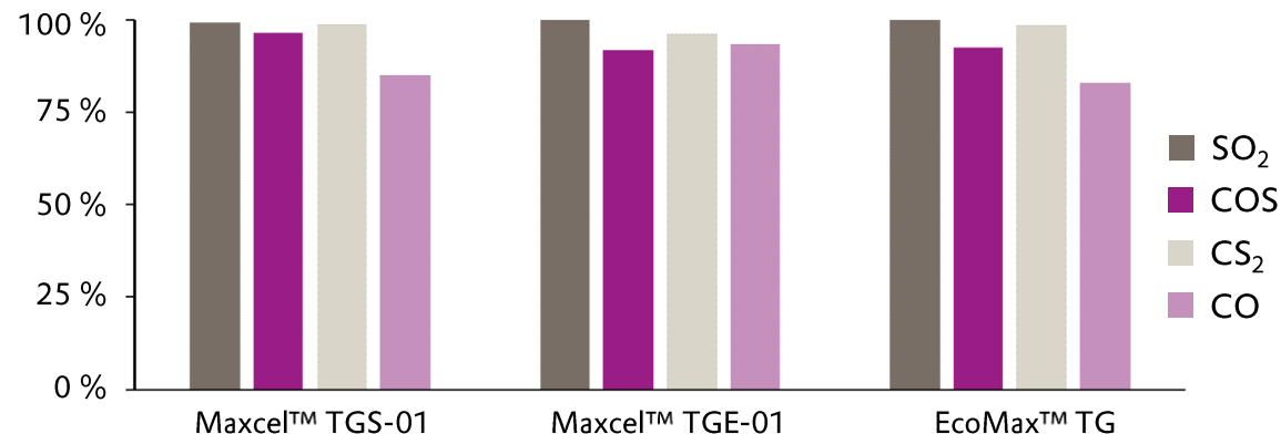
Conversion in Tail Gas Reactor - Conventional - 1200 GHSV / 280°C bed temperature
