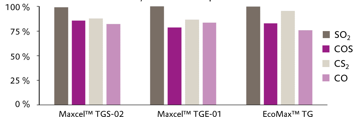
Conversion in Tail Gas Reactor - Low Temperature - 1200 GHSV / 240°C bed temperature
